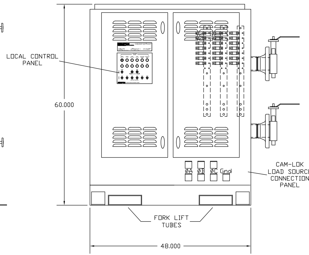
FRONT VIEW
