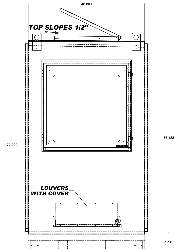
RIGHT VIEW
