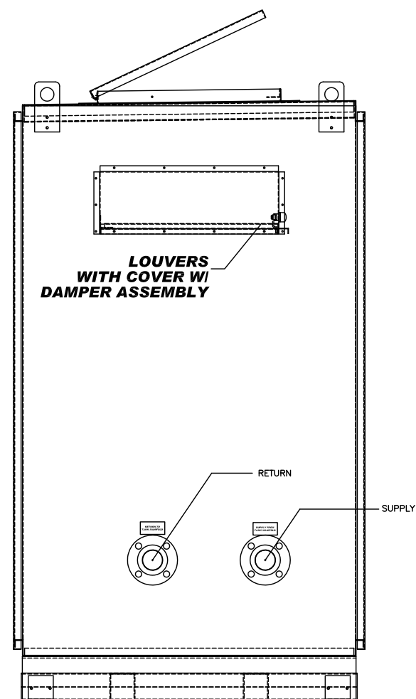
LEFT VIEW
