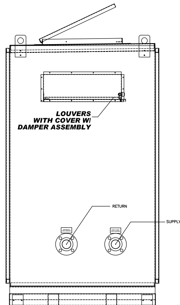
LEFT VIEW
