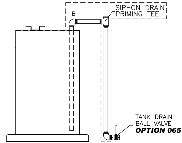
SIPHON DRAIN DETAIL
