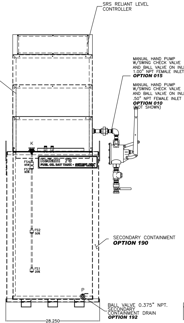
FRONT VIEW
