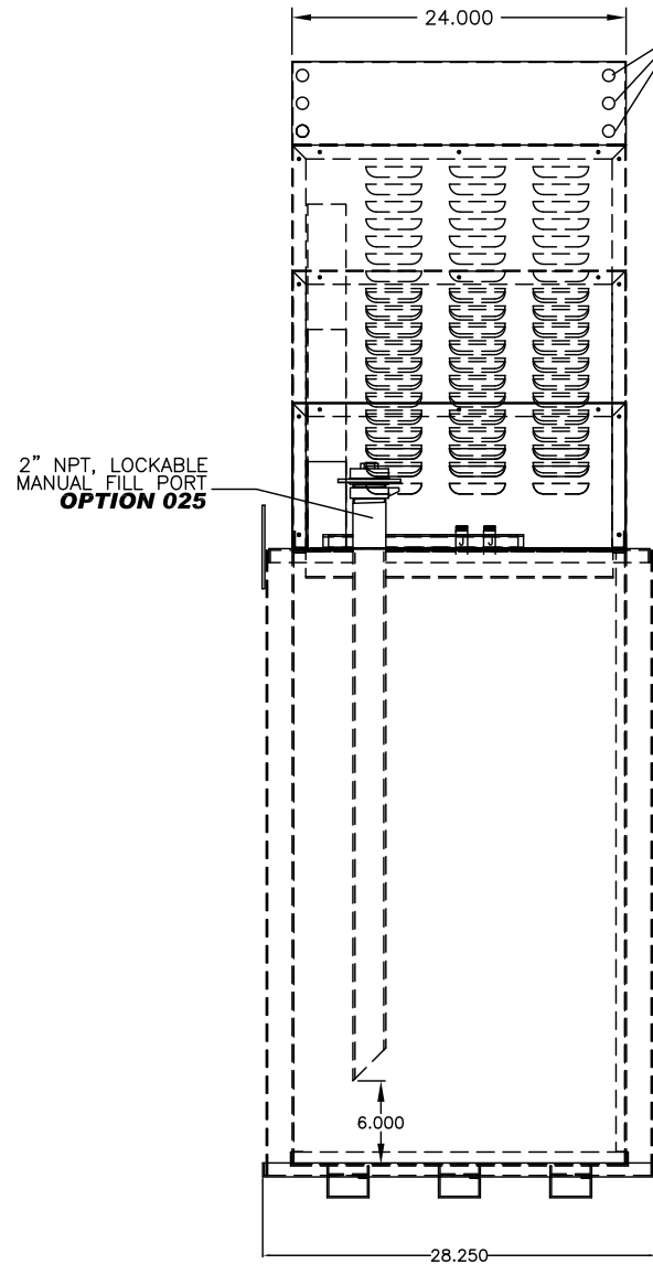
REAR VIEW
