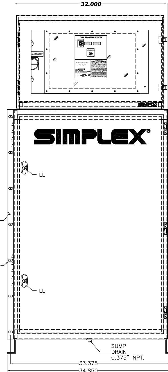
FRONT VIEW
