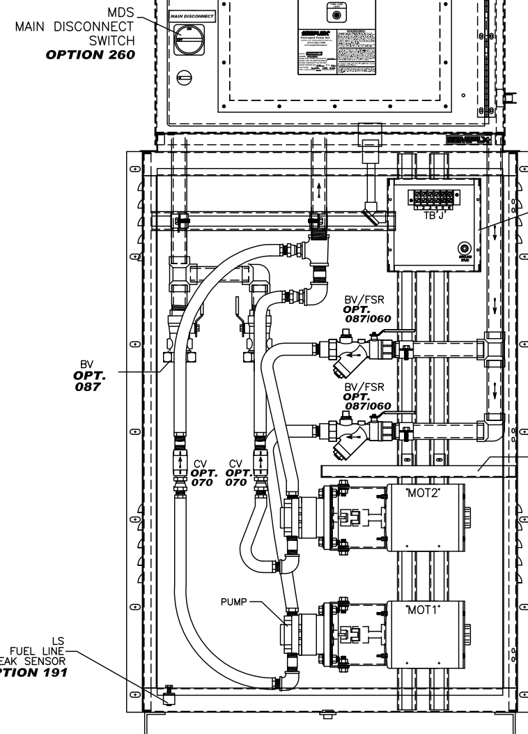
ENCLOSURE SHOWN WITHOUT DOORS
