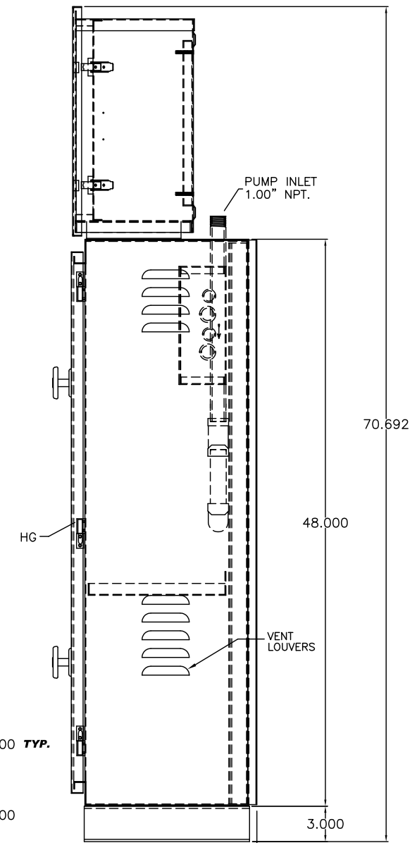
RIGHT SIDE
