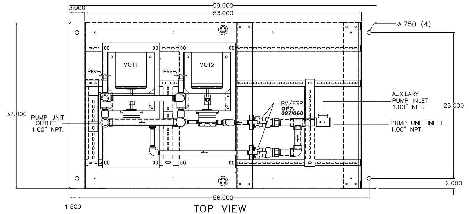
PIPING DIAGRAM
