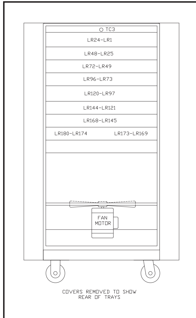
Part of Typical Tray Layout Drawing
