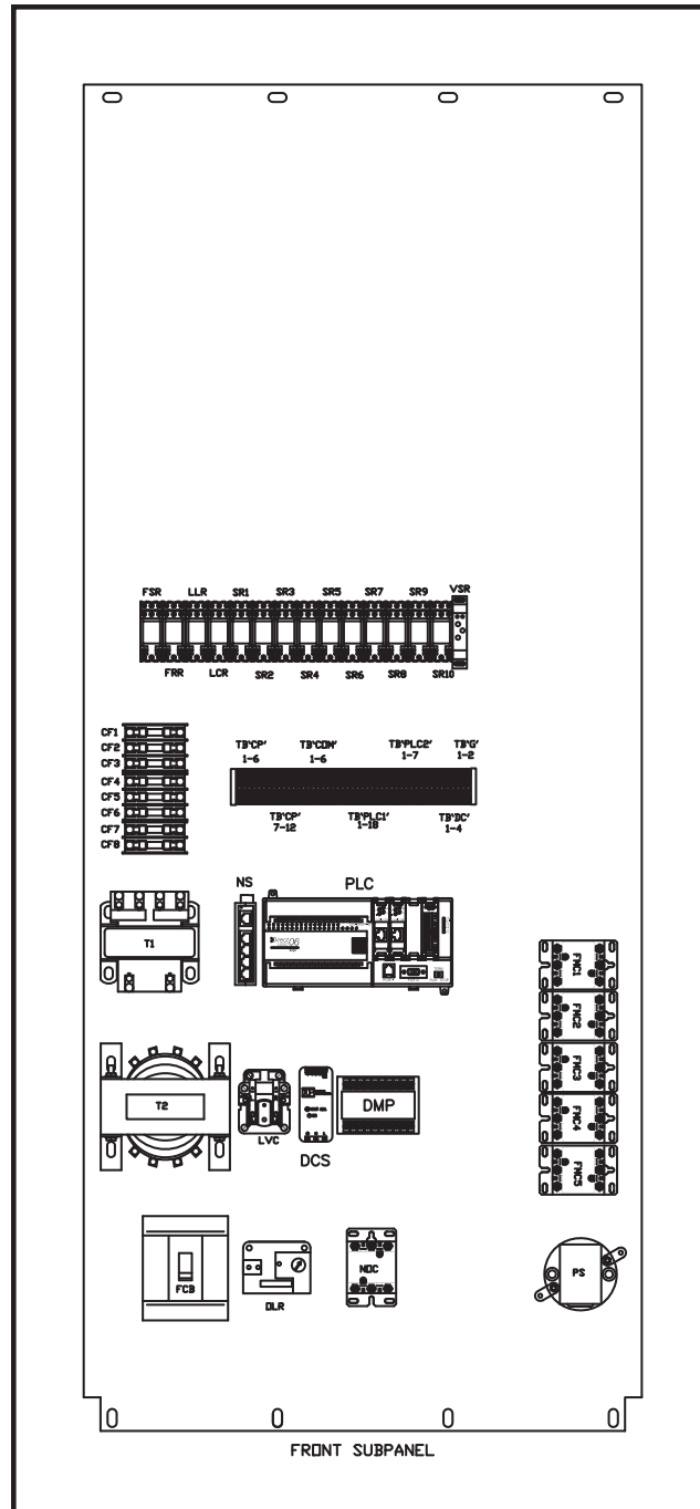
Part of Typical Subpanel Drawing
