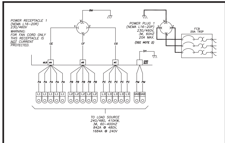
Part of Typical Power Distribution Drawing
