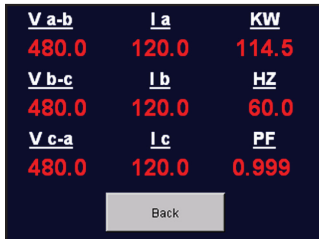
Metering Screen
