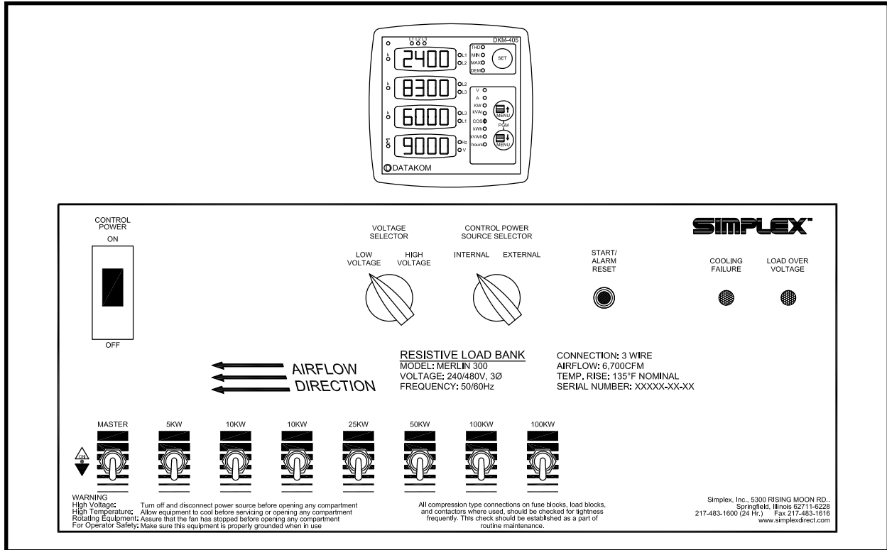
Part of Typical Local Control Detail Drawing
